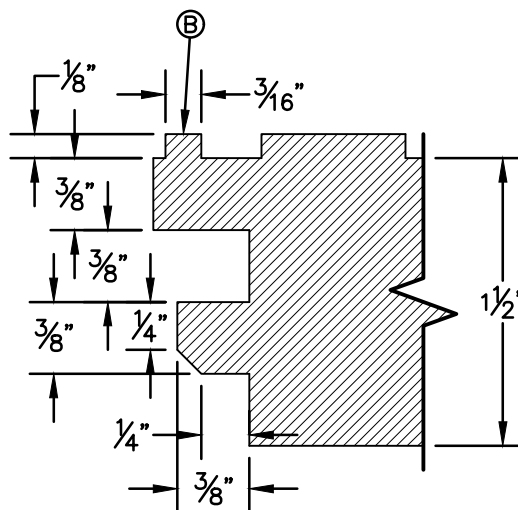
LOCKING TAB DETAIL
